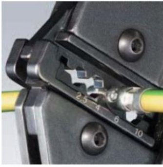
Crimp System Pliers 97 43 200 with crimping dies 94 49 30 for non-insulated butt connectors
